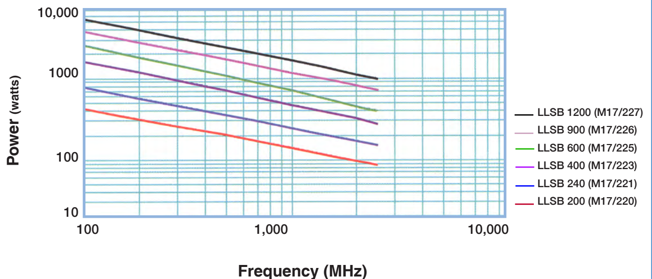
Power Handling vs. Frequency (Typical)
