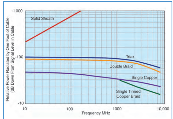
Fig. 9 Shielding Effectiveness
