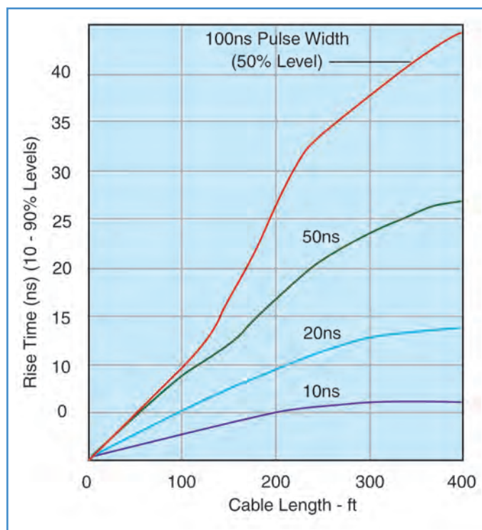
Fig. 11 Pulse Distortion
