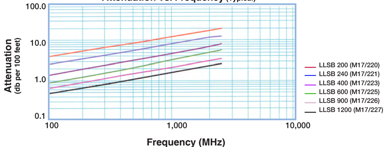
Attenuation vs. Frequency (Typical)
