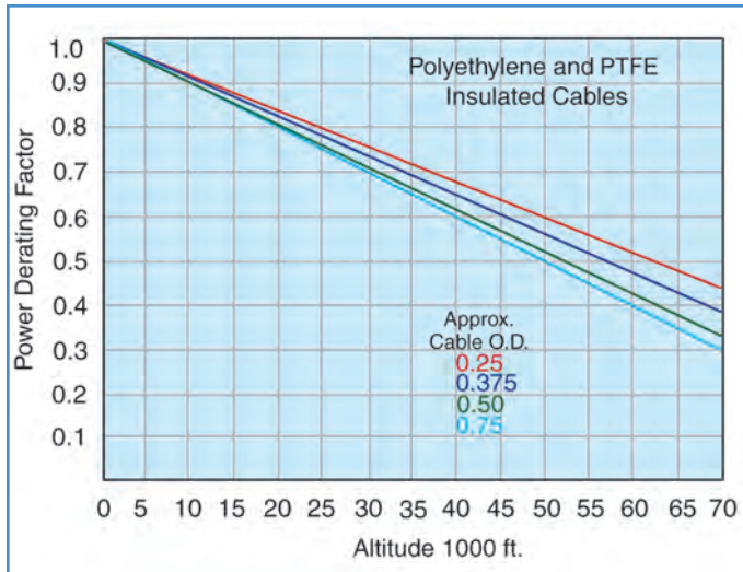
Fig. 7 Power Altitude Correction Factor
